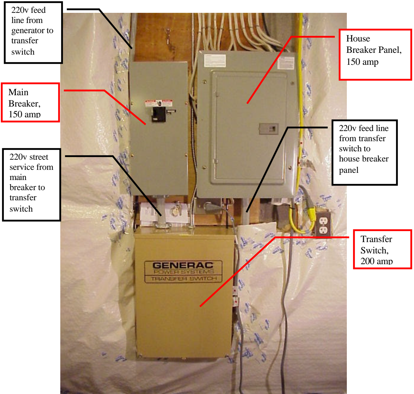
Electrical Panels & Transfer Switch Detail
